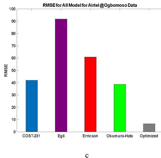
Figure 6: (a) Path Loss against Distance for LAUTECH Main gate, Ogbomosho Airtel Base Station (b) Standard Deviation graph (c) Root Mean Square Error (RMSE) graph.
